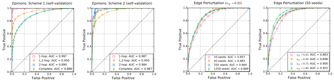
Figure 6: Epinions (self-validation): ROC curves for both schemes
